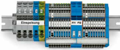
FI main distribution board set TOPJOB® S; with operating slots
