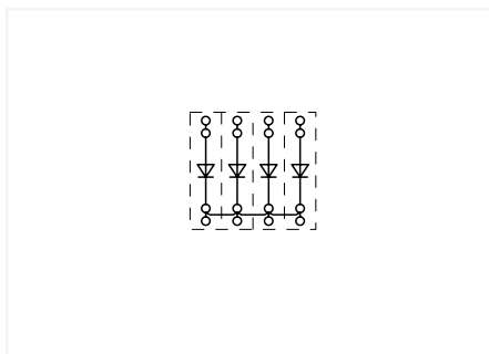
Polarized diode gates with a common cathode can be created using the following terminal blocks: 279-815/281-410 or 279-815/281-411
