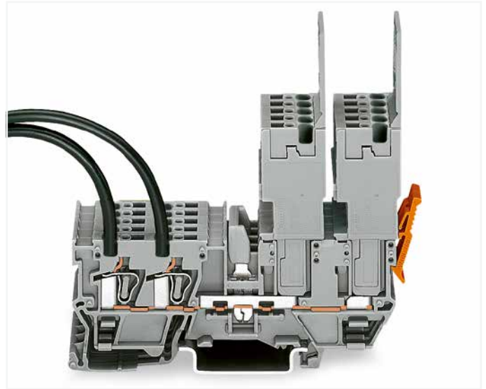
2 x 1-conductor female plugs Carrier terminal blocks can be commoned via 280 and 780 Series Jumpers and tested using a test plug adapter (280-4..).
