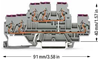
91 mm/3.58 in
