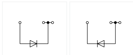
3-conductor diode terminal block; with 1N4007 diode; gray
