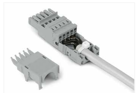
2- to 5-pole strain relief housings feature one cable outlet (rear side). 6- to 7-pole strain relief housings feature one cable outlet 8- to 9-pole strain relief housings feature two cable outlets and one cover. 10- to 16-pole strain relief housings feature three cable outlets and two covers.
