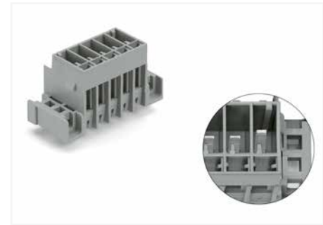
Male header; with preceding contact; with straight solder pins and mounting flanges
