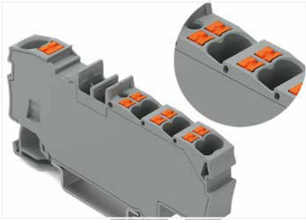
A clear marking of clamping units is molded in.
