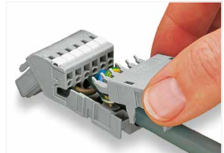
Snapping on a strain relief housing.
