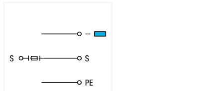
Actuator terminal block; with ground connection; for fuse plugs; for phase protection; without end plate
