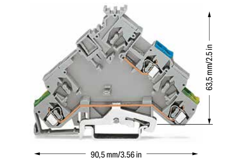
Actuator terminal block; with ground connection; with 1N4007 recovery diode
