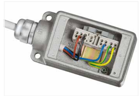
Wiring example in an Ex junction box
