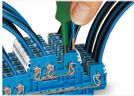
CAGE CLAMP® termination: Inserting a conductor via operating tool (0.08 ... 4 mm 2 "f-st").
