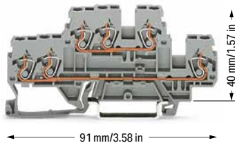
91 mm/3.58 in
