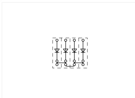
Polarized diode gates with a common cathode can be created using the following terminal blocks: 279-673/281-410 or 279-673/281-411
