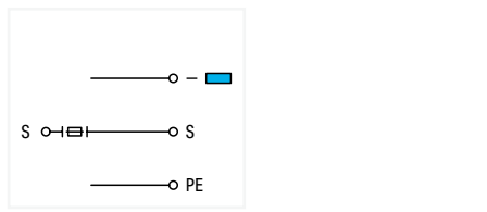
Actuator terminal block; with ground connection; for fuse plugs; for phase protection; with end plate
