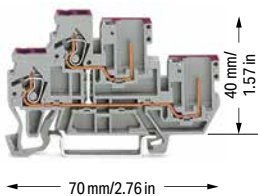
2-conductor/2-pin double-deck carrier terminal block; 2-conductor/2-pin through terminal block; internally commoned; Violet conductor entry; gray
