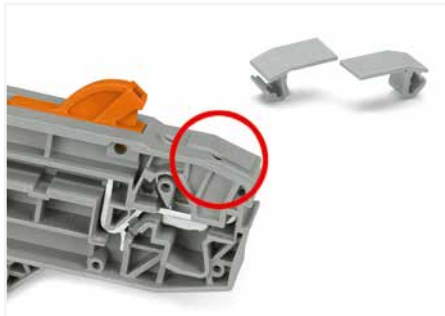
Cover (2006-191) seals unused conductor entry.
