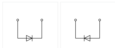
2-conductor diode terminal block; with 1N4007 diode; gray
