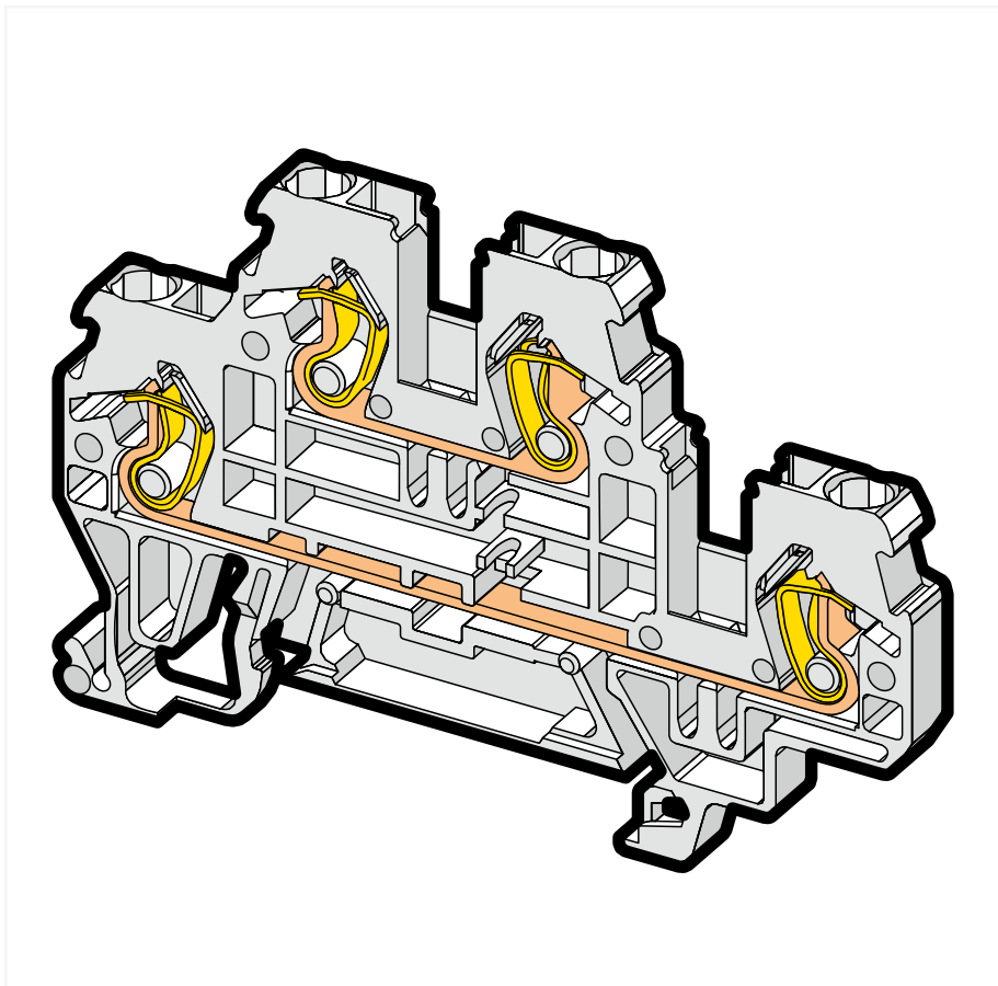
CAGE CLAMP® termination: Inserting a conductor via operating tool (0.08 ... 4 mm 2 "f-st"). With ferruled conductors, it is necessary to use a terminal block one size smaller than the conductor's nominal cross section.
