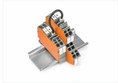
Push-in type wire jumpers common terminal blocks over longer distances and across multiple levels.
