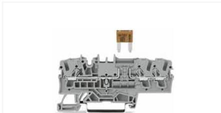
Fuse terminal blocks for mini-automotive blade-style fuses
