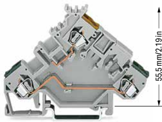
80 mm / 3.15 in 55,5 mm / 2.19 in 280-555 280-554
