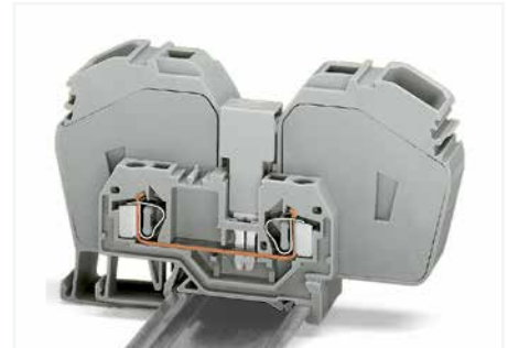
Commoning a 285 Series terminal block (35 mm 2 / 2 AWG) with a 281 Series terminal block (4 mm 2 / 12 AWG) using a step-down jumper (283-414).
