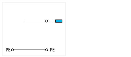
Actuator supply terminal block; with ground connection; power supply from actuator side
