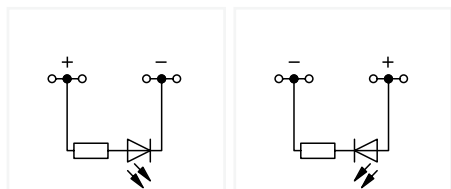
4-conductor LED terminal block; with red LED; gray
