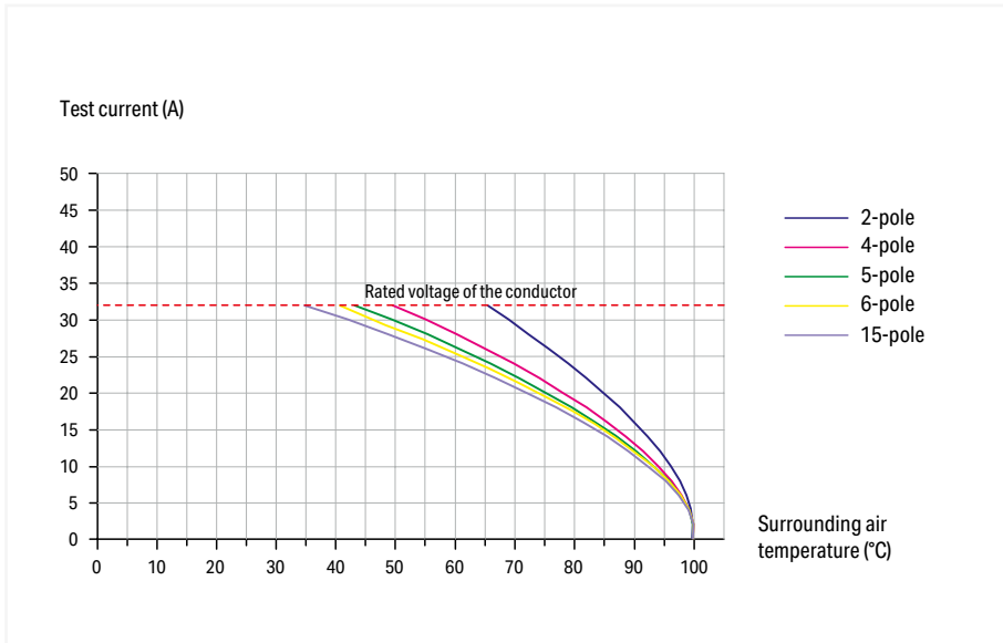
Male connectors with CAGE CLAMP® connection (769-602 to 769-615) Conductor cross section: 4 mm² (12 AWG)
