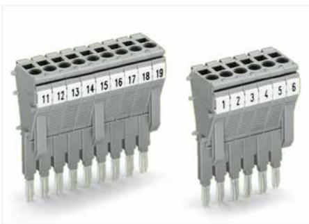
Using anti-reverse mating modules at both ends of a module assembly prevents reverse mating.
